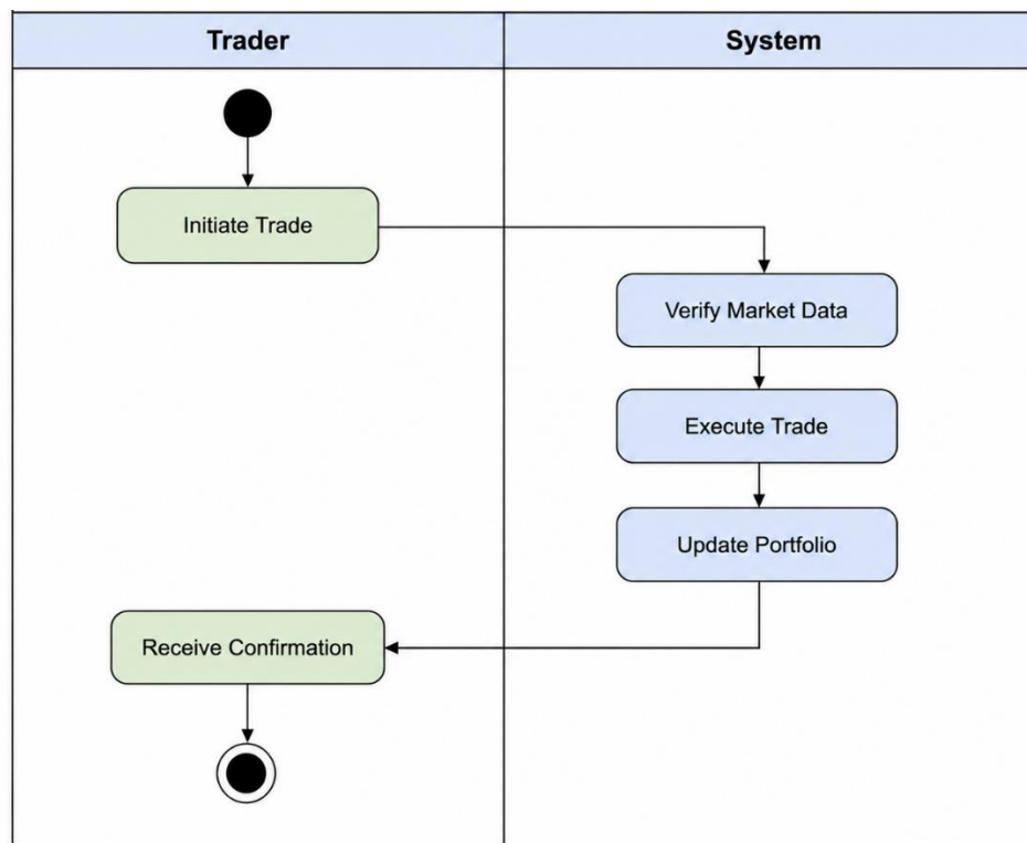
Activity Diagram 2 – Execute Trade
