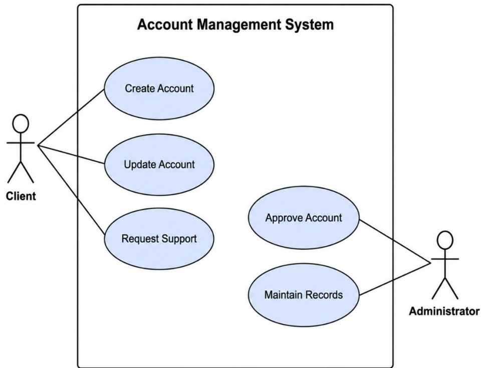
Use Case Diagram 2 – Client Account Management
