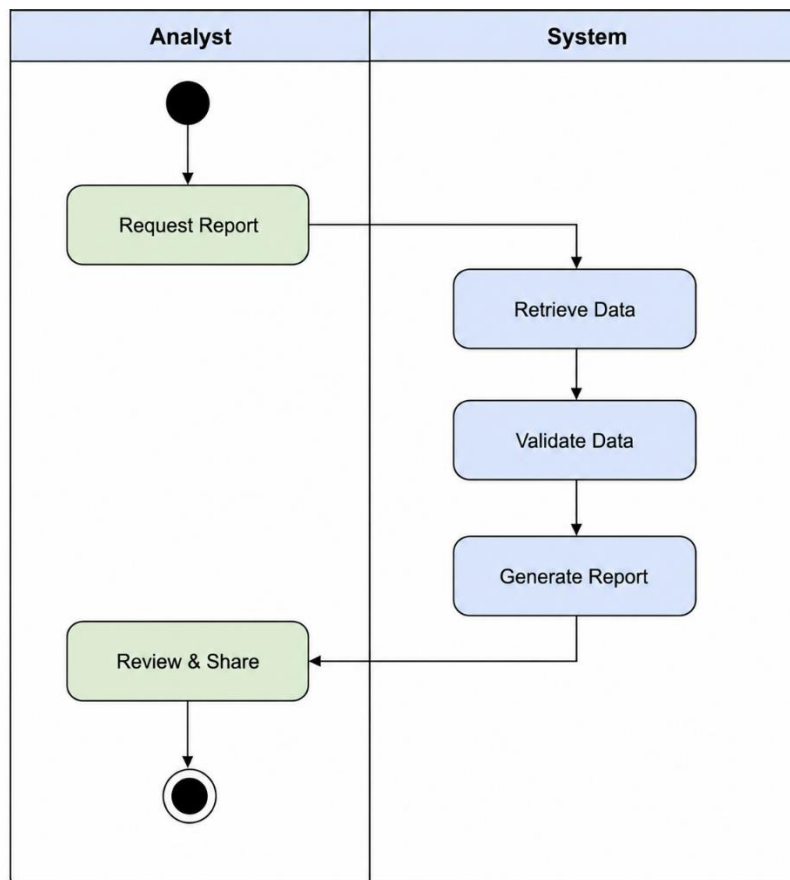
Activity Diagram 1 – Generate Automated Report
